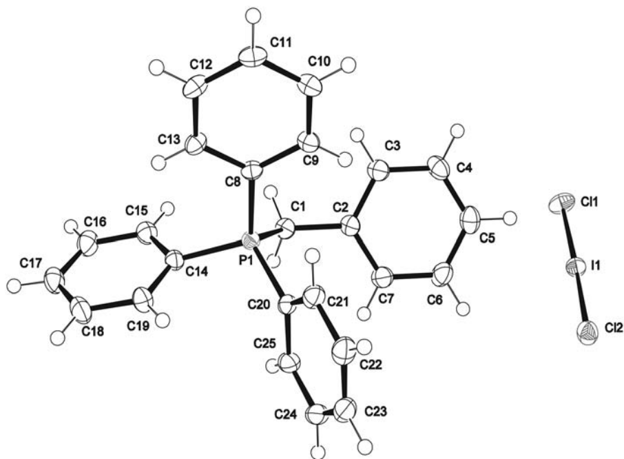
Fig. 1. ORTEP Drawing of the molecule structure of \text{BnPh}_3\text{P}^+(\text{ICl}_2)^-
