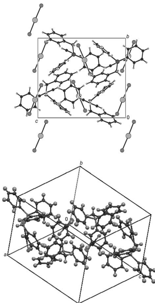
Fig. 2. Two views of the unit cell of BnPh_3P^+(ICl_2)^-
